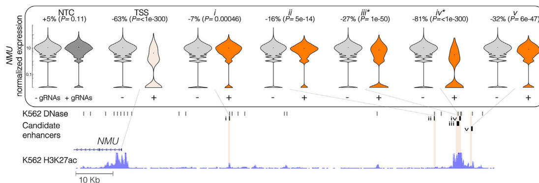
Figure 5. Highlighted Examples of Enhancer-Gene Pairs
